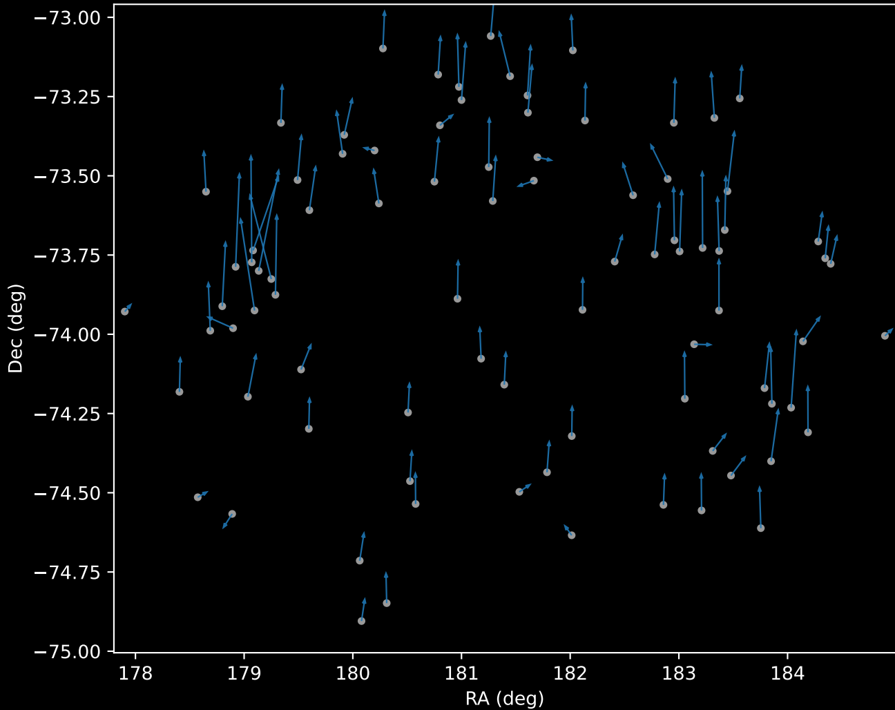
GALAH DR4 Cluster 0 Proper Motion Vectors (n=86)
