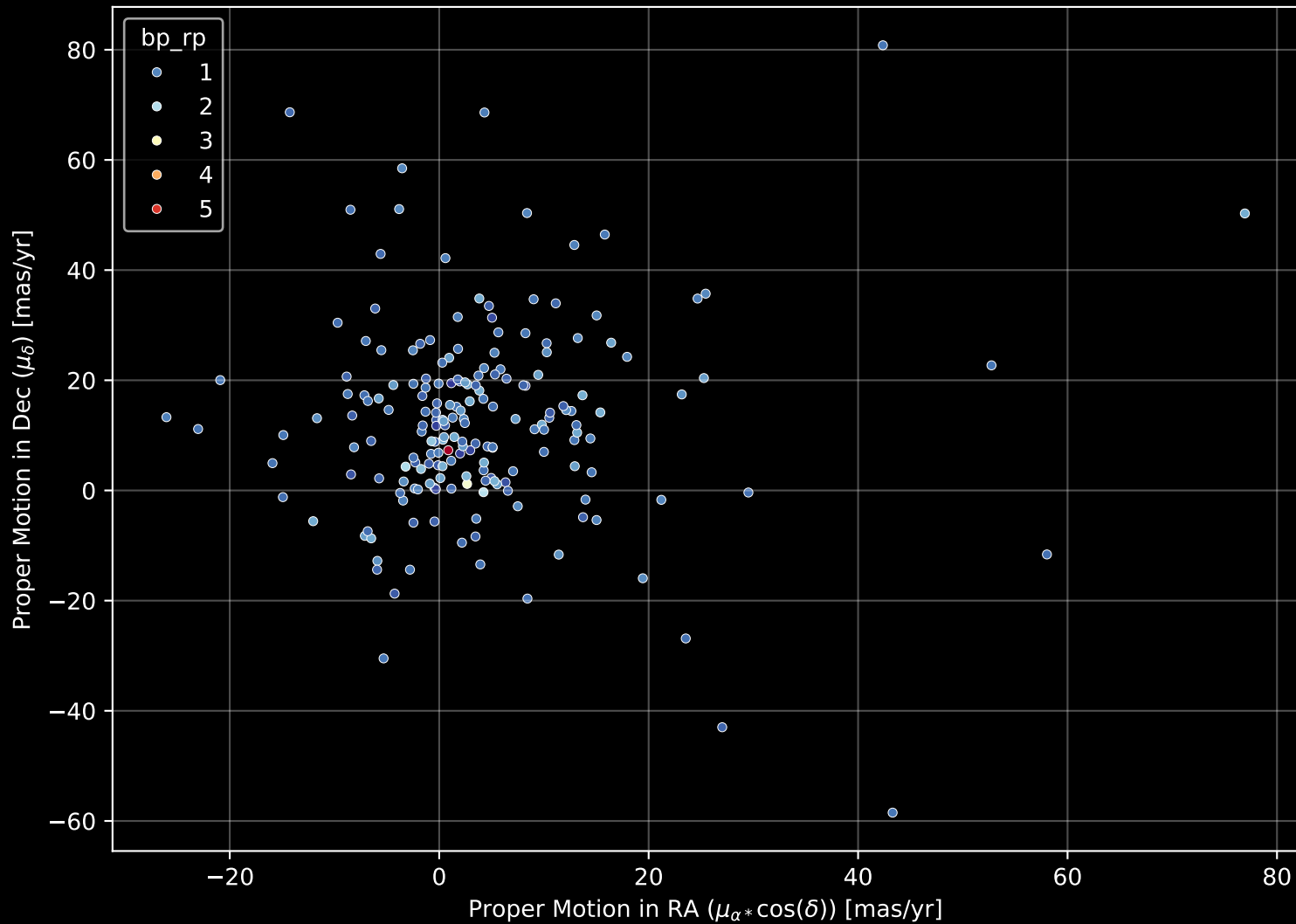
GALAH DR4 Field: [7174] Proper Motion Diagram (n= 192)
