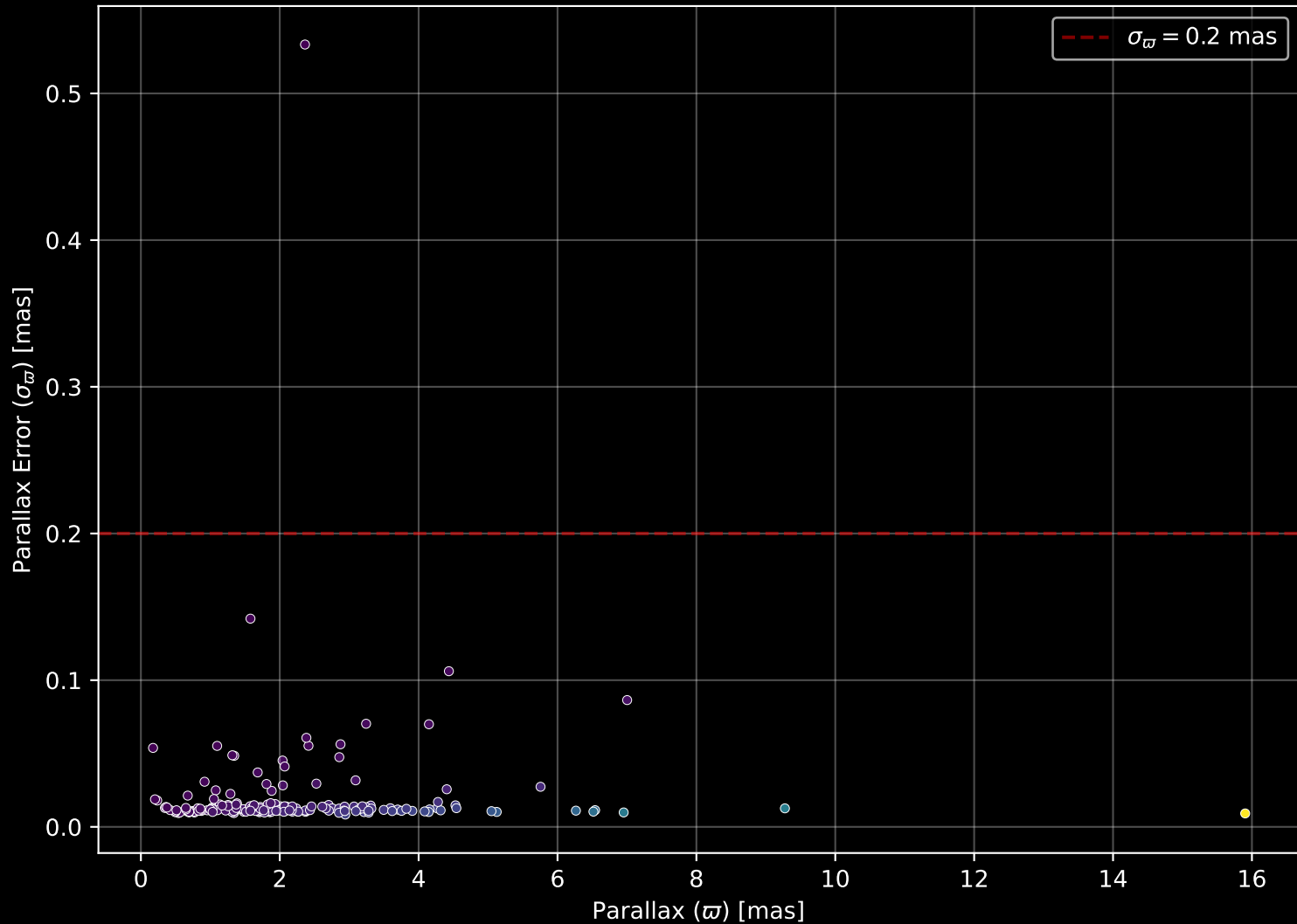
GALAH DR4 Field: [7174] Parallax Quality (n= 192)
