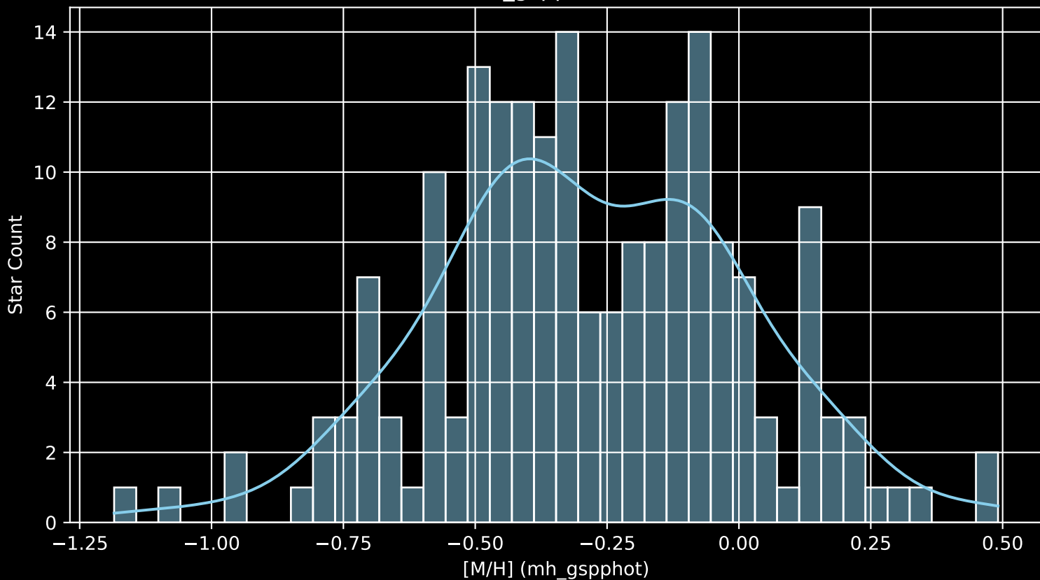
GALAH DR4 Field: [7174] [M/H] (mh_gspphot) (n= 190)
