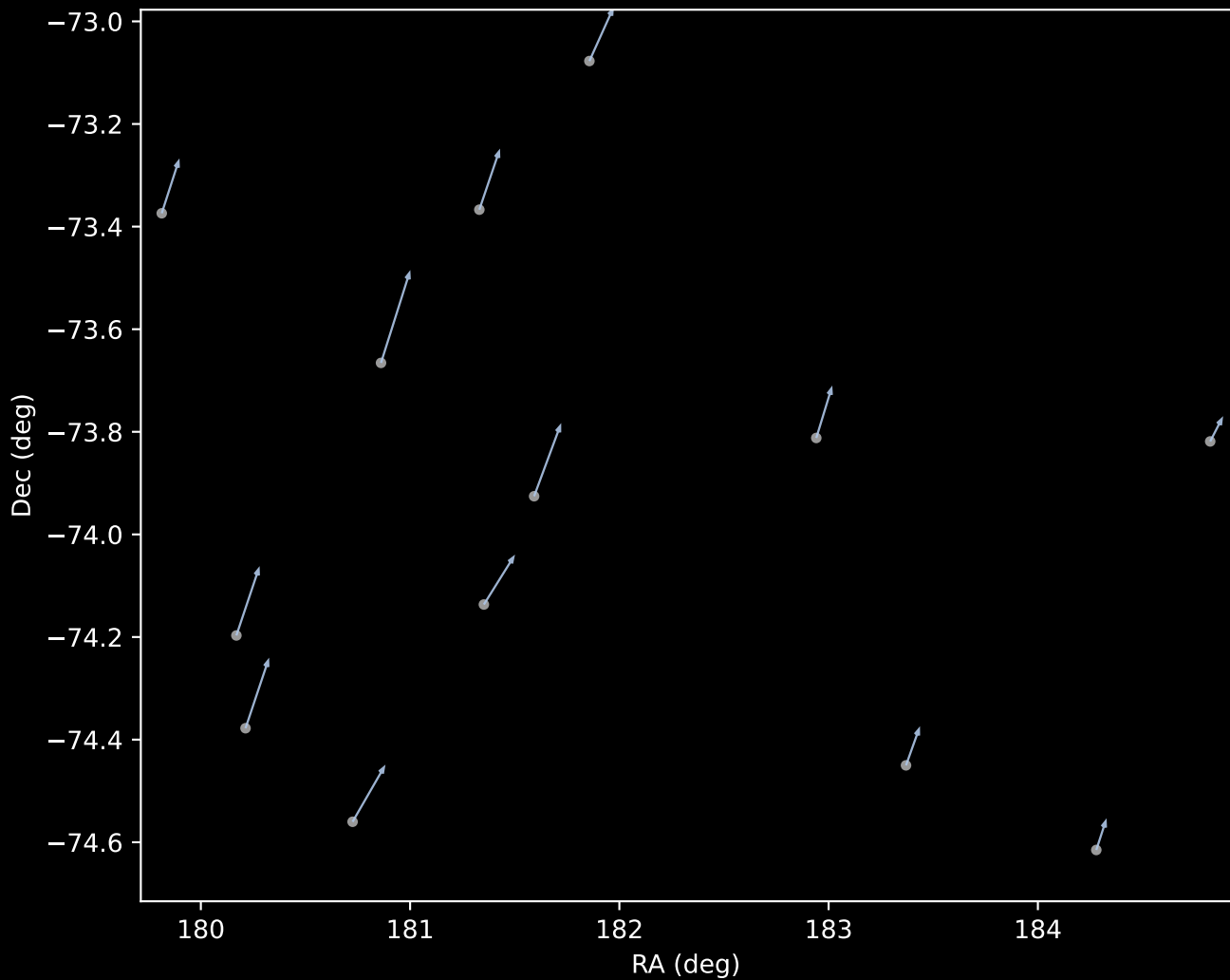
GALAH DR4 Cluster 1 Proper Motion Vectors (n=13)
