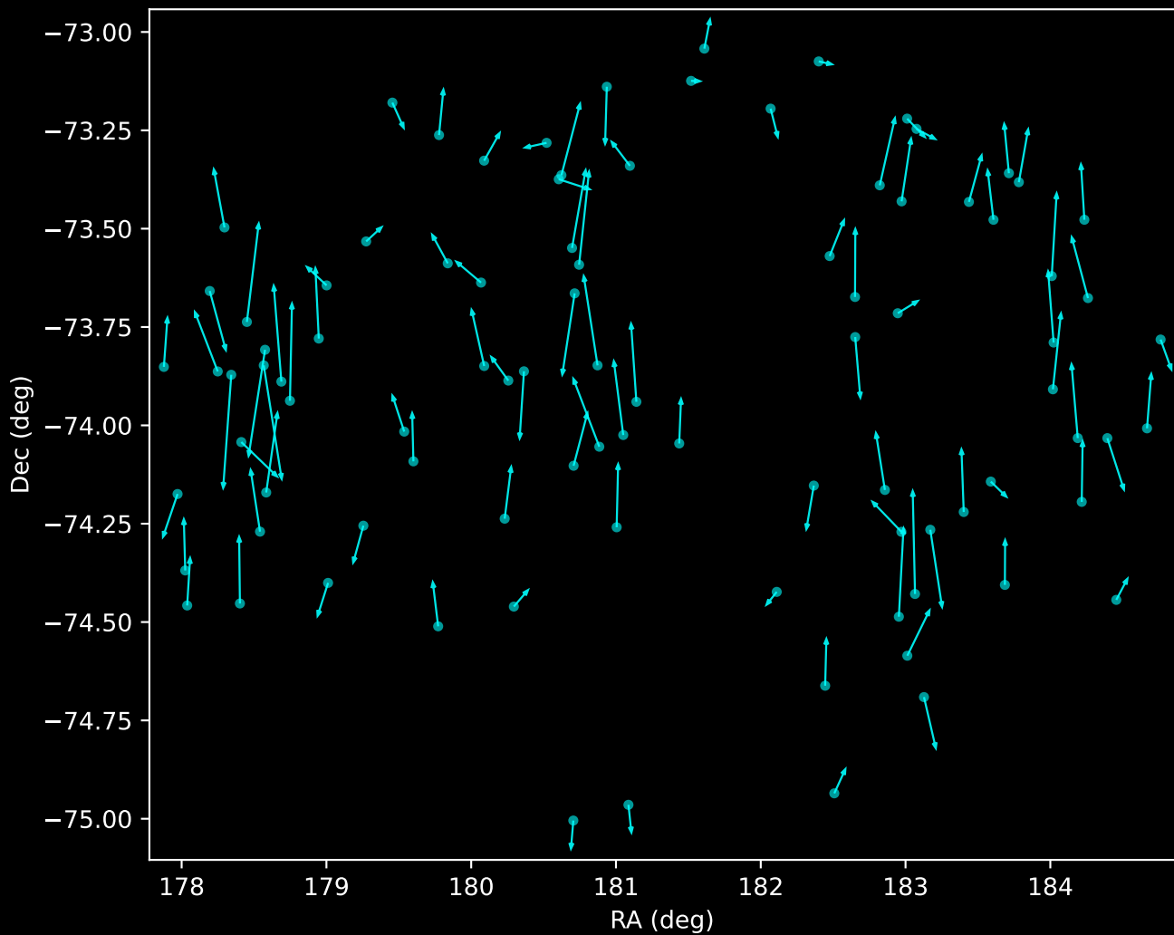
GALAH DR4 Noise Stream Proper Motion Vectors (n=93)
