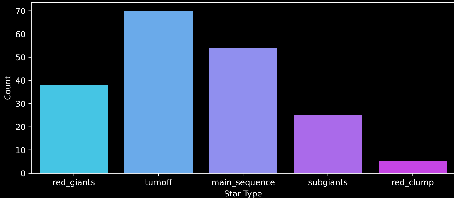
GALAH DR4 Field: [7174] Count plot of Star Type
