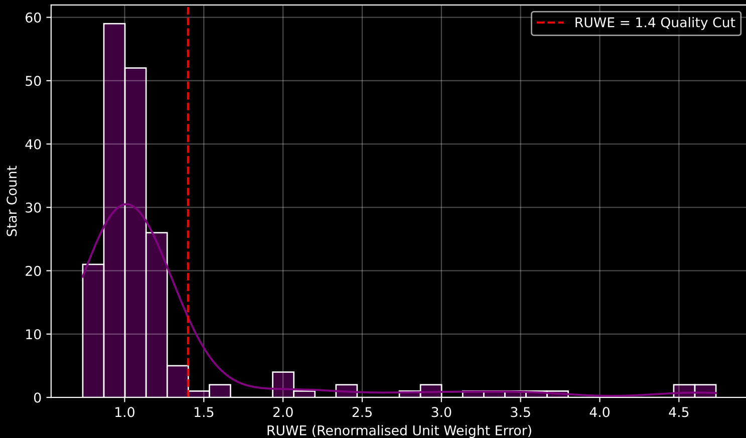
GALAH DR4 Field [7174] RUWE Distribution (n= 185)
